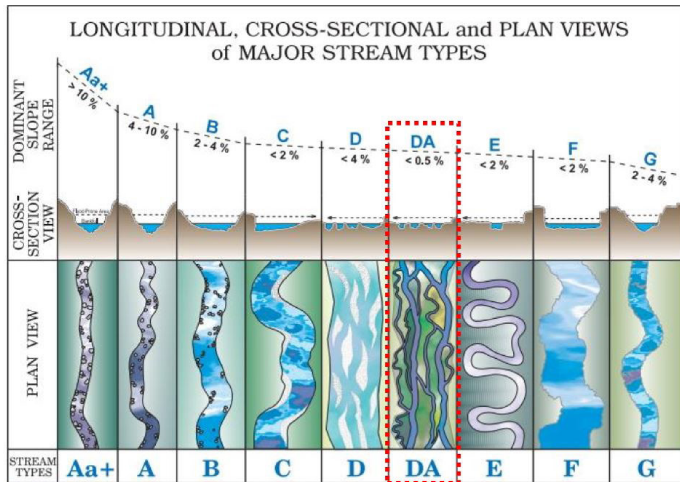
Figure A-1. Broad-level stream classification delineation showing longitudinal, cross-sectional and plan views of major stream types (Rosgen, 1994, 1996).
